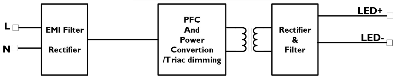
LED Driver Circuit Block Diagram
