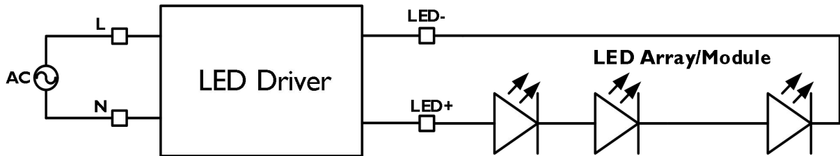
Wiring Diagram
